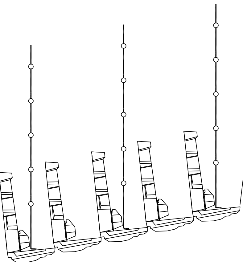
1:5 WALL BATTER
