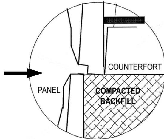
ASSEMBLY DETAIL
